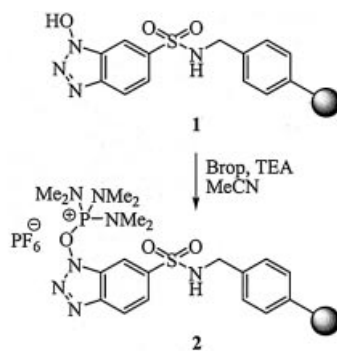
Scheme 1. Synthesis of P-BOP ( 2 )
