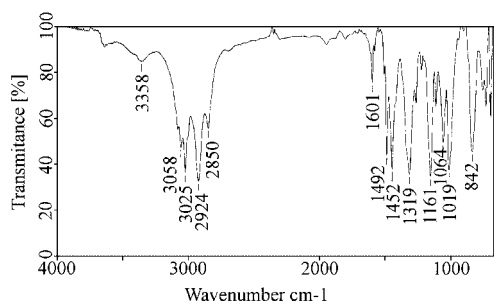
Figure 1. The IR spectra of P-BOP (2)
