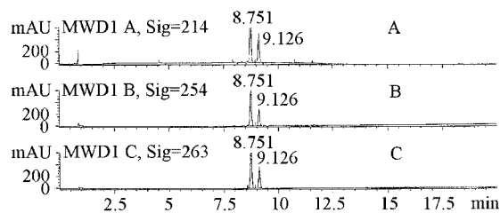
Figure 2. The HPLC chromatogram of the crude reaction mixture resulting after the coupling between 3 and 4 , in dichloromethane and using pyridine as base, at \lambda = 214 (A), 254 (B) and 263 nm (C), respectively
